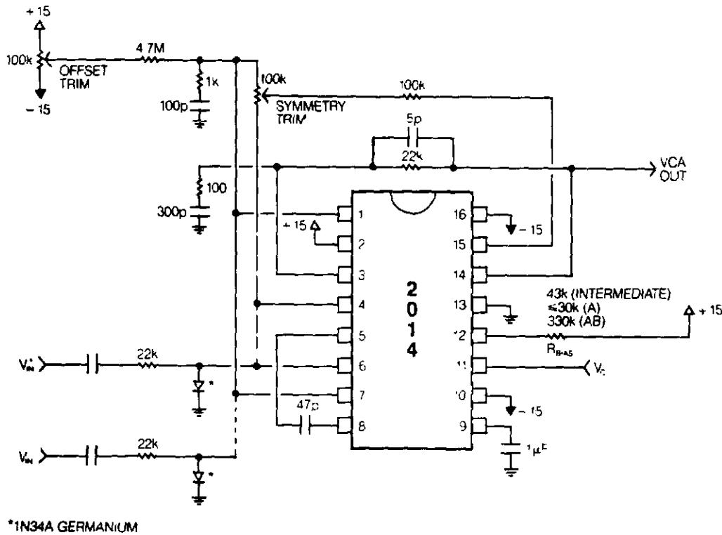
FIGURE 4. MINIMUM VCA (DIFFERENTIAL INPUTS)
