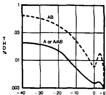
ONE CHANNEL ( V_o or V_{i,a} ) VCP GAIN dB
