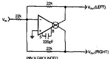
INVERTING
