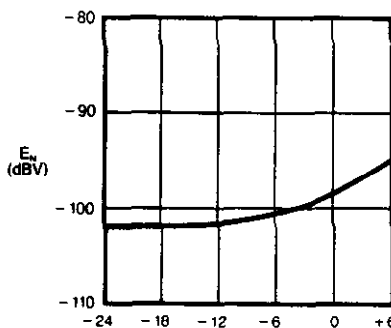
GAIN (dB)
