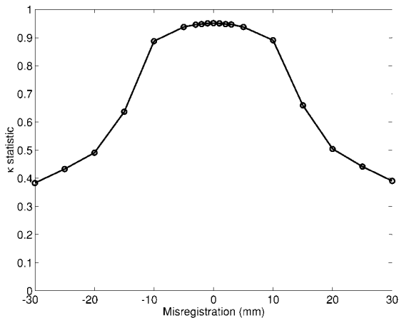
FIG. 5. Segmentation accuracy with respect to misregistration with the a priori images.
