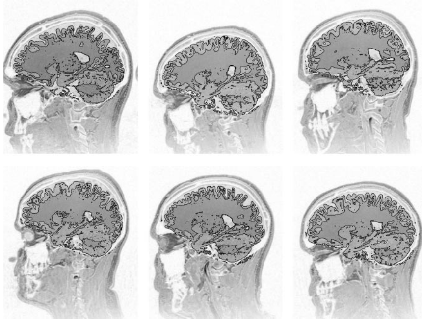
FIG. 2. A single sagittal slice through six T1-weighted images (2-T scanner, with an MPRAGE sequence, 12^\circ tip angle, 9.7 ms repeat time, 4 ms echo time, and 0.6 ms inversion time). Contours of extracted gray and white matter are shown superimposed on the images.
